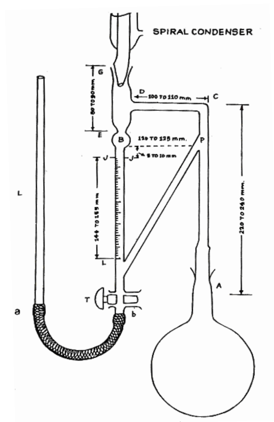
Fig. Apparatus for volatile oil determination
